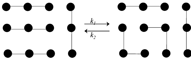
Figure 8. An illustration of the suggested change in the distribution of \text{Ag}-\text{Ag} bonded [\text{Ag}(\text{CN})_2^-]_n excitons upon laser irradiation. The increased number of bent trimer excitons concomitant with a decrease in the number of linear trimer excitons in the forward reaction (the writing process) should lead to a higher HE/LE intensity ratio, as observed experimentally.
