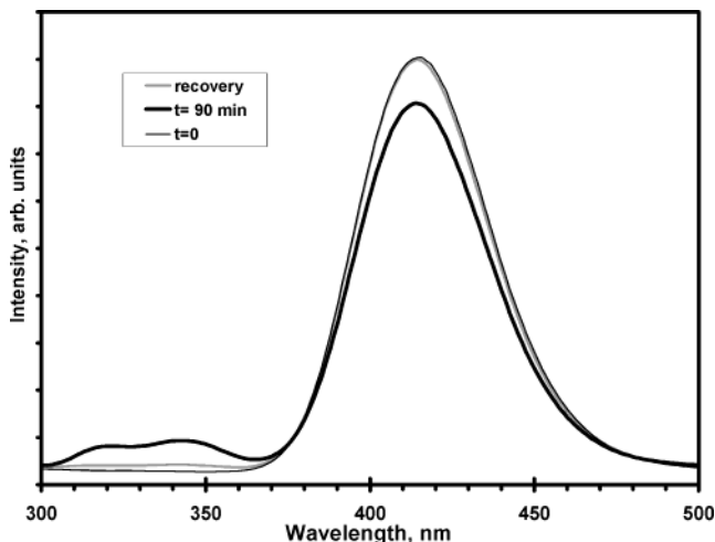
Figure 3. Emission spectra versus 266 nm laser irradiation time at 77 K for pure \text{KAg}(\text{CN})_2 crystals. All spectra were scanned with 275 nm excitation. Note the appearance of the short-wavelength bands following irradiation at 77 K and their quenching in the recovery step after the sample is heated to ambient temperature and then cooled again to 77 K.
