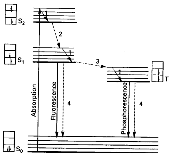
Figure 1 The Jablonski diagram. Radiative and non-radiative processes are depicted as solid and dashed lines, respectively.
