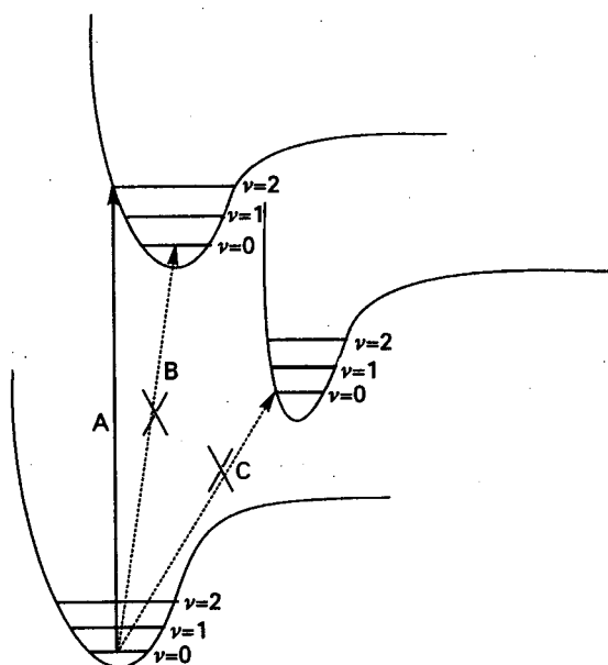
Figure 2 The Franck-Condon principle. Only vertical electronic transitions are allowed.
