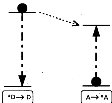
Figure 15 Phonon-assisted energy transfer. The energy difference between the excited states of D and A is provided by phonons.
