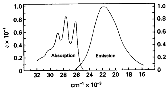
Figure 8 Emission (right) and absorption (left) spectra of cyclohexyl-9-anthroate in benzene. Reproduced with permission from Shon RS-L, Cowan DO and Schmiegell WW (1975) Photodimerization of 9-anthroate esters and 9-anthramide. The Journal of Physical Chemistry 79: 2087–2092.
