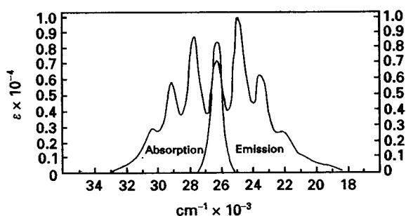
Figure 7 Emission (right) and absorption (left) spectra of 9-anthramide in tetrahydrofuran. Reproduced with permission from Shon RS-L, Cowan DO and Schmiegell WW (1975) Photodimerization of 9-anthroate esters and 9-anthramide. The Journal of Physical Chemistry 79: 2087–2092.
