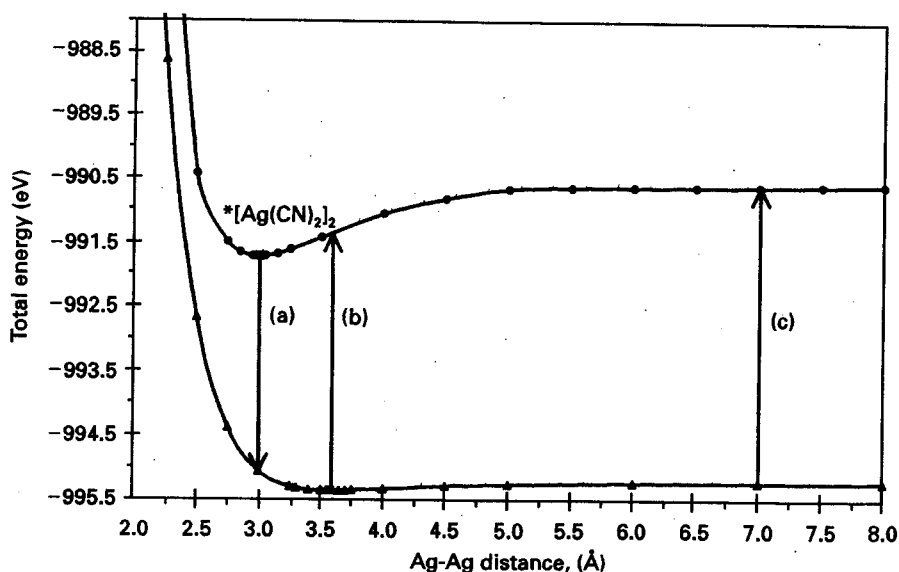
Figure 21 Potential energy diagram of the ground and the first excited electronic states of [\text{Ag}(\text{CN})_2]_2 (eclipsed configuration) as plotted from extended Hückel calculations. The excimer [\text{Ag}(\text{CN})_2]_2 corresponds to the potential minimum of the excited state. The optical transitions shown are (a) excimer emission, (b) solid state excitation and (c) dilute solution absorption. (Reproduced with permission from Omary MA and Patterson HH (1998) Luminescent homoatomic exciplexes in dicyanoargentate (I) ions doped in alkali halide crystals: 1. Exciplex tuning by site-selective excitation. Journal of the American Chemical Society 120: 7696–7705.
