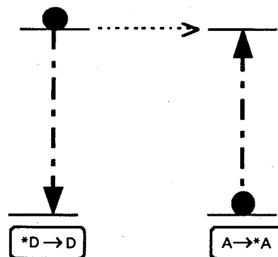
Figure 14 Energy transfer from a donor (D) to an acceptor (A).
