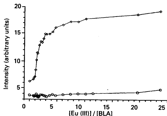
Figure 17 Luminescence titration of apo- \alpha -lactalbumin (BLA) with europium chloride in D_2O . The luminescence intensity is monitored for the ^5D_0 \rightarrow ^7F_2 emission line of Eu(III) with \lambda_{exc} = 395 nm. The upper curve shows the data for BLA-bound Eu(III) and the lower curve shows the data for EuCl_3 alone. Reproduced with permission from Bünzli JCG and Choppin GR (1989) Lanthanide Probes in Life, Chemical and Earth Sciences , p 279. Amsterdam: Elsevier.
