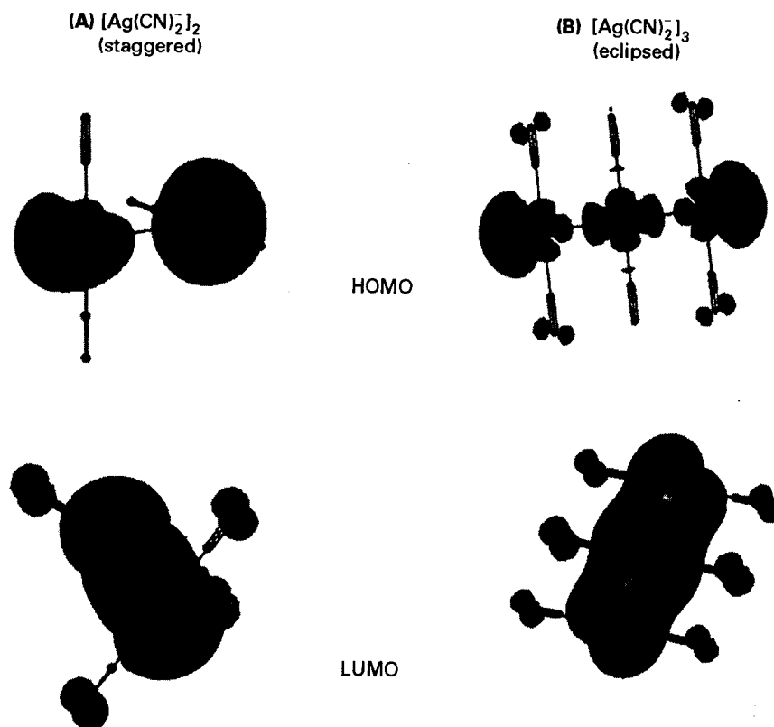
Figure 22 Surfaces of the highest occupied molecular orbital (HOMO) and the lowest unoccupied molecular orbital (LUMO) for [\text{Ag}(\text{CN})_2]_2 (staggered isomer) and [\text{Ag}(\text{CN})_2]_3 (eclipsed isomer), as plotted from ab initio calculations. Note the Ag–Ag antibonding character for the HOMO and the Ag–Ag bonding character for the LUMO in both cases.
