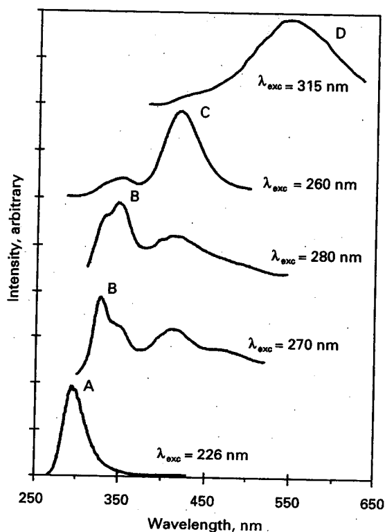
Figure 20 Photoluminescence spectra of [\text{Ag}(\text{CN})_2]^-/\text{KCl} doped crystals at 77 K. The letter assignment of the luminescence bands follows the notation used in Table 2. Reproduced with permission from Omary MA and Patterson HH (1998) Luminescent homoatomic exciplexes in dicyanoargentate (I) ions doped in alkali halide crystals: 1. Exciplex tuning by site-selective excitation. Journal of the American Chemical Society 120: 7696–7705.
