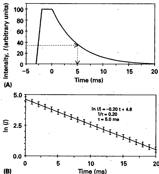
Figure 5 Experimental determination of excited state lifetimes: (A) a plot of the intensity ( I ) versus time after the laser pulse. The lifetime corresponds to the time at which the intensity decays to 1/e of its maximum value; (B) a plot of \ln(I) versus time after laser pulse. The lifetime here can be calculated directly from the slope of the linear equation.
