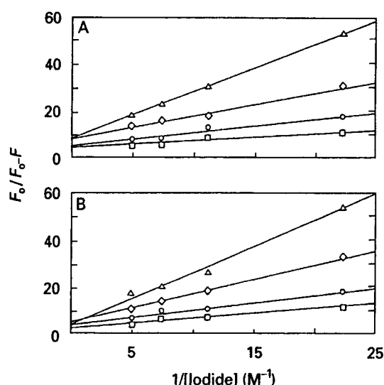
Figure 13 A modified Stern–Volmer plot for the fluorescence quenching of HDL 1 by iodide in the presence of varying amounts of acrylamide. The data are shown for HDL 1 samples obtained from rats fed with manganese-deficient (top) and manganese-adequate (bottom) diet. The fluorescence was monitored at 338 nm ( \lambda_{exc} = 295 nm) characteristic of tryptophan residues. Reproduced with permission from Taylor PN, Patterson HH and Klimis-Tavatzis DJ (1997) A fluorescence double-quenching study of native lipoproteins in an animal model of manganese deficiency. Biological Trace Element Research 60: 69–80.
