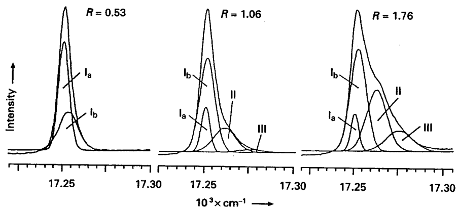
Figure 18 Curve-resolved Eu(III) excitation spectra of apo-BLA in D_2O . R represents the [Eu(III)]/[BLA] ratio. Reproduced with permission from Bünzli JCG and Choppin GR (1989) Lanthanide Probes in Life, Chemical and Earth Sciences , p 280. Amsterdam: Elsevier.
