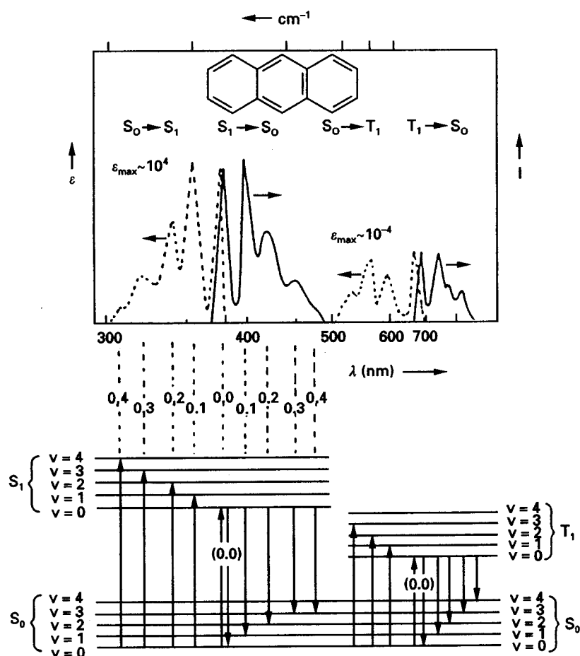
Figure 6 Emission (solid line) and absorption (dashed line) spectra of anthracene in solution. The assignments of the vibronic transitions are shown in the bottom portion of the figure. Reproduced with permission from Turro NJ (1978) Modern Molecular Photochemistry , p 94. Menlo Park: Benjamin/Cummings.
