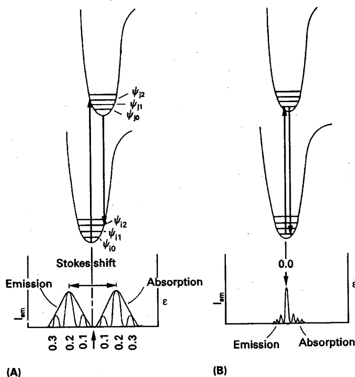
Figure 3 Potential energy diagrams for two cases of excited state distortions: (A) non-zero distortion and (B) zero distortion. The corresponding absorption and emission spectra are shown below. Reproduced with permission from Adamson AW and Fleischauer PD (1975) Concepts of Inorganic Photochemistry , p 4. New York: Wiley-Interscience.
