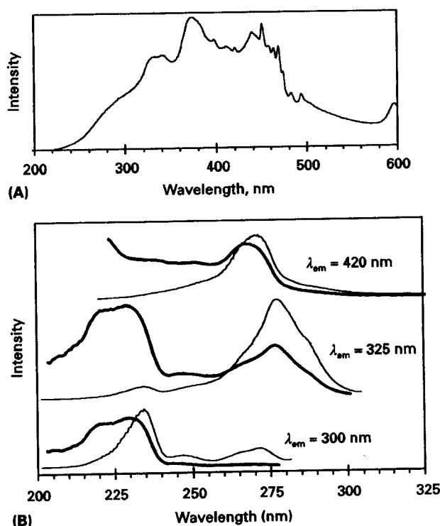
Figure 4 Correction of the excitation spectra by the quantum counter method: (A) excitation spectrum of rhodamine B; (B) excitation spectra of [\text{Ag}(\text{CN})_2]^-/\text{NaCl} doped crystals monitoring the emission at different wavelengths. Corrected and uncorrected spectra are shown as thick and thin lines, respectively.
