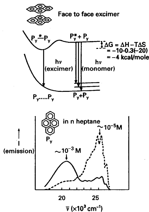
Figure 19 Excimer emission of pyrene. The upper curves show the potential surfaces of the ground and the luminescent excited electronic state (Reproduced with permission from Turro NJ (1978) Modern Molecular Photochemistry , p 141. Menlo Park: Benjamin/Cummings.
