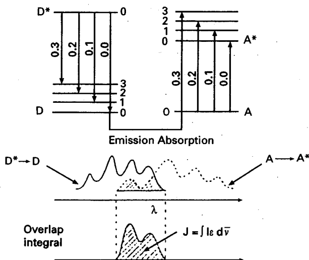
Figure 16 Experimental determination of the donor–acceptor spectral overlap from emission and absorption spectra. Reproduced with permission from Turro NJ (1978) Modern Molecular Photochemistry , p 299. Menlo Park: Benjamin/Cummings.
