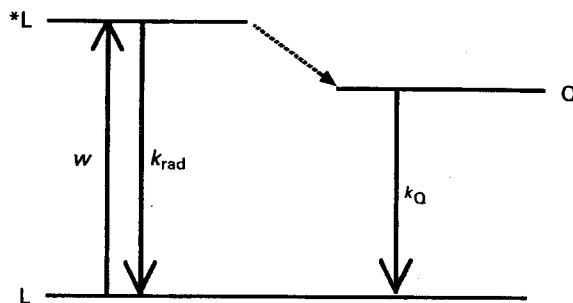
Figure 11 Kinetic model for dynamic quenching. In the notation used w , k_{rad} and k_Q refer to the absorption rate, radiative rate and quenching rate, respectively.
