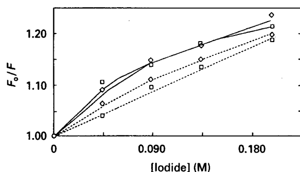
Figure 12 A Stern–Volmer plot for the fluorescence quenching of HDL 1 (solid lines) and HDL 2 (dashed lines). The different legends refer to samples obtained from rats fed with manganese-adequate (◊) and manganese-deficient (◻) diet. The fluorescence was monitored at 338 nm ( \lambda_{exc} = 295 nm) characteristic of tryptophan residues. (Reproduced with permission from Taylor PN, Patterson HH and Klimis-Tavatzis DJ (1997) A fluorescence double-quenching study of native lipoproteins in an animal model of manganese deficiency. Biological Trace Element Research 60: 69–80.
