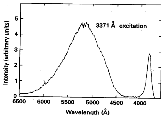
Figure 9 Luminescence spectrum of \text{BaPd}(\text{CN})_4 \cdot 4\text{H}_2\text{O} at 7 K. A nitrogen laser was used for excitation. Reproduced with permission from Ellenson WD, Viswanath AK and Patterson HH (1981) Laser-excited luminescence study of the chain compound \text{BaPd}(\text{CN})_4 \cdot 4\text{H}_2\text{O} . Inorganic Chemistry 20: 780–783.
