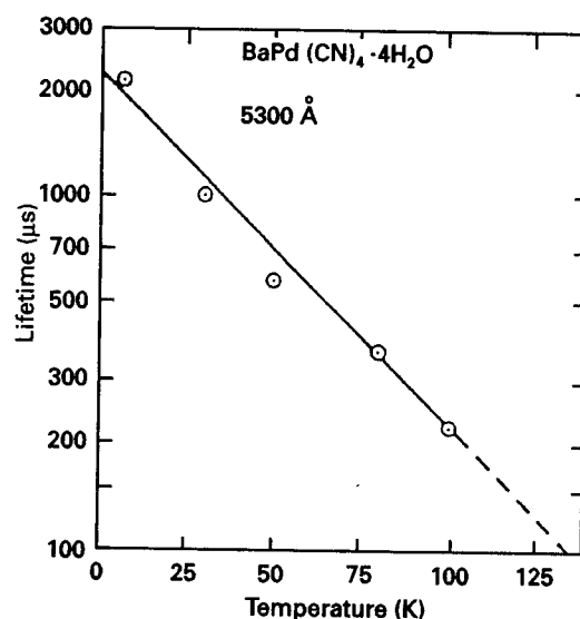
Figure 10 Lifetime of the 19 \times 10^3 \text{ cm}^{-1} luminescence band of \text{BaPd}(\text{CN})_4 \cdot 4\text{H}_2\text{O} versus temperature. The dashed line is extrapolation to higher temperatures. Reproduced with permission from Ellenson WD, Viswanath AK and Patterson HH (1981) Laser-excited luminescence study of the chain compound \text{BaPd}(\text{CN})_4 \cdot 4\text{H}_2\text{O} . Inorganic Chemistry 20: 780–783.
