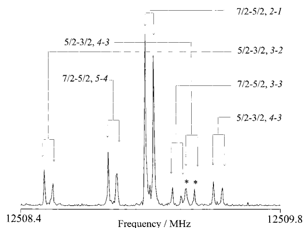
Figure 2. Hyperfine structure in the J = 4-3 transitions of ^{16}\text{O}^{12}\text{C}^{65}\text{Cu}^{35}\text{Cl} and ^{16}\text{O}^{12}\text{C}^{65}\text{Cu}^{37}\text{Cl} (indicated with an asterisk). Experimental conditions: 0.1% \text{Cl}_2 , 1.5% CO in argon, 1000 averaging cycles, 4K data points, 4K transform. Quantum numbers F_{\text{Cu}}'-F_{\text{Cu}}'' ; F'-F'' .
